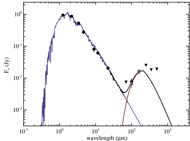
Figure 2. SED for LP 876-10. Dots are fluxes and triangles 3\sigma upper limits. Black symbols are measured fluxes and grey symbols are star-subtracted (i.e. disc) fluxes. The 3200K stellar photosphere model is shown in blue, the 24K blackbody disc model in red, and the star+disc spectrum in black.
