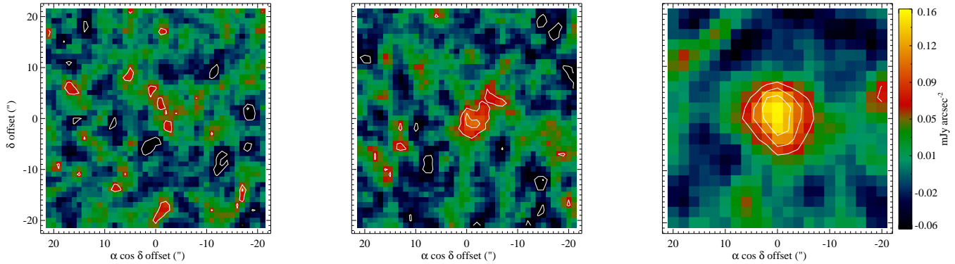
Figure 1. Herschel PACS images of LP 876-10, at 70, 100 and 160 \mu\text{m} from left to right. The expected December 2010 source position of \alpha = 22\text{h } 48\text{m } 4.7\text{s} , \delta = -24^\circ 22\text{m } 9.9\text{s} is at the centre of the images, and the PACS pointing accuracy for these observations is about 2 arcseconds at 1\sigma . Contours are drawn at intervals of \pm 2, 3 and 4\sigma .
