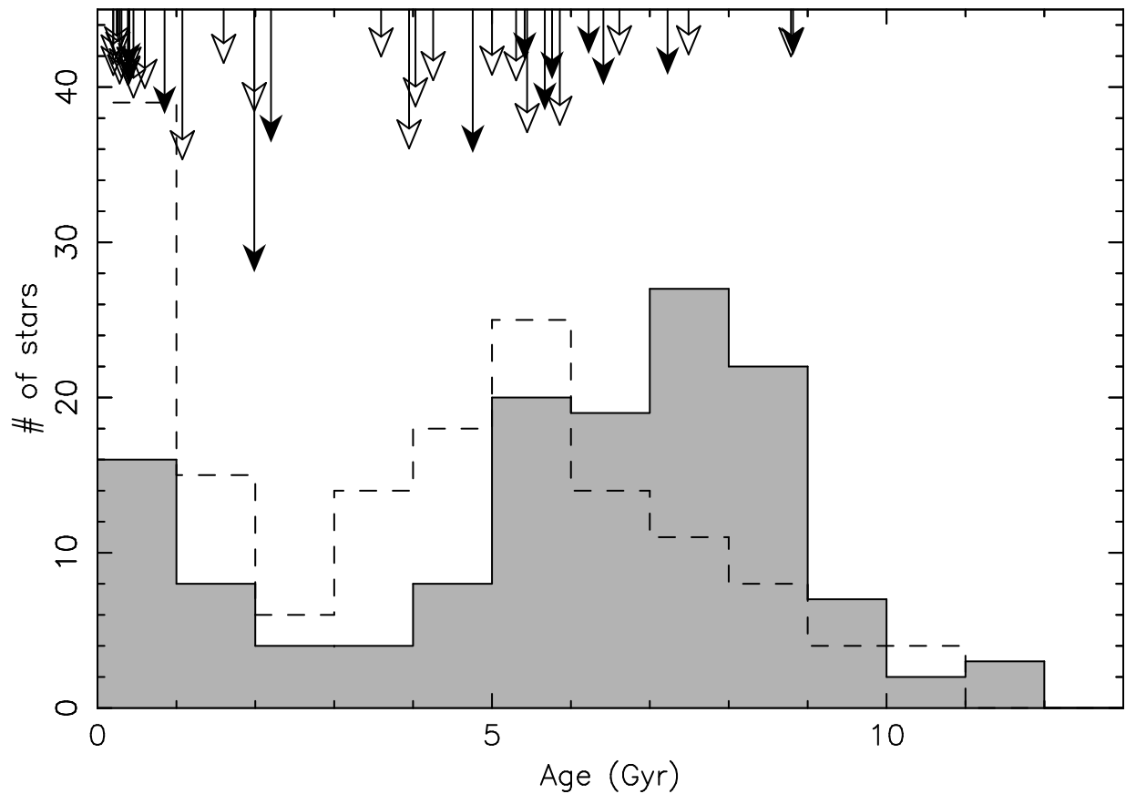
Fig. 2.— Estimated ages for the observed stars. The ages for the planet-bearing stars are shown as a filled histogram, while those for the control sample of stars not known to have planets are outlined with a dashed line. The ages of stars with 70 \mu\text{m} excess are flagged as arrows at the top of the plot, with the length of each arrow proportional to the strength of the excess emission. Solid arrows indicate IR excess stars known to have planets while open arrows correspond to stars in the control sample.
