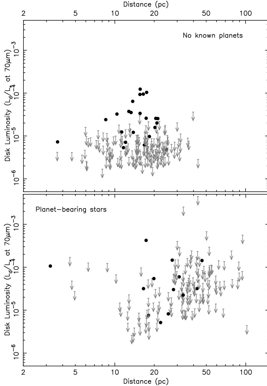
Fig. 1.— Debris disk fractional luminosities for stars without known planets (upper panel) and for stars with planets (lower panel) as a function of stellar distance. For stars with significant excess (solid points), a minimum L_{\text{dust}}/L_{\star} is derived from the strength of the 70 \mu\text{m} emission relative to the stellar photosphere (eq 2). Otherwise, 3 \sigma upper limits are shown, again based solely on the 70 \mu\text{m} emission. (Note that the planet-bearing star HD 69830 has a large 24 \mu\text{m} excess, but for self-consistency its L_{\text{dust}}/L_{\star} is shown here as an upper limit based solely on its 70 \mu\text{m} emission.) Overall, the planet-bearing stars tend to be farther away and have not been limited to clean regions of the sky, making it more difficult to detect faint emission around them.
