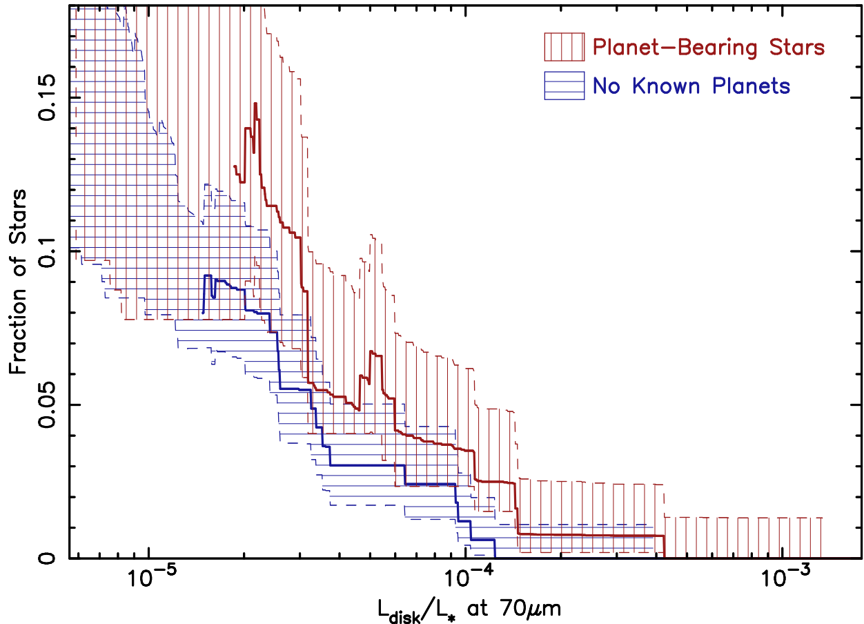
Fig. 3.— The cumulative fraction of stars with 70\ \mu\text{m} excess as a function of disk luminosity for the planet and non-planet samples. As in figure 1, the dust’s fractional luminosity, L_{\text{dust}}/L_{\star} , is derived from the strength of the 70\ \mu\text{m} emission relative to the stellar photosphere (eq 2). For both the planet and non-planet samples, dust disks with L_{\text{dust}}/L_{\star} > 10^{-4} are rare, with L_{\text{dust}}/L_{\star} \approx 10^{-5} disks detected much more frequently. The 1\ \sigma uncertainties in the underlying distributions of L_{\text{dust}}/L_{\star} are indicated by the shaded regions. While the dust around planet-bearing stars is nominally brighter than for the non-planet stars (i.e. the red line lies above the blue line), the difference is not statistically significant.
