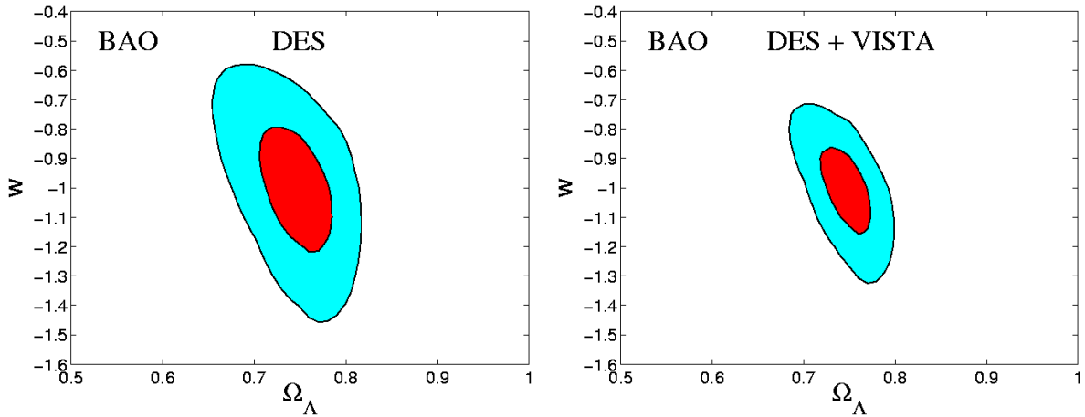
Figure 1: The expected 1\sigma (red) and 2\sigma (blue) likelihood contours for w (the equation of state of DE) versus \Lambda for just the DES (LEFT) and VDES (RIGHT) detections of the BAOs. These constraints are based on large N -body simulations. For the DES case, we assume 5000 sq degrees with z_{max} = 1.3 and 10 redshift bins of dz = 0.13 . VDES simulation is the same area but with z_{max} = 1.7 and 22 redshift bins of dz = 0.08 . The background cosmological model in the simulations has \sigma_8 = 0.9 , \Omega_k = 0 , \Omega_b = 0.044 , and h = 0.7
