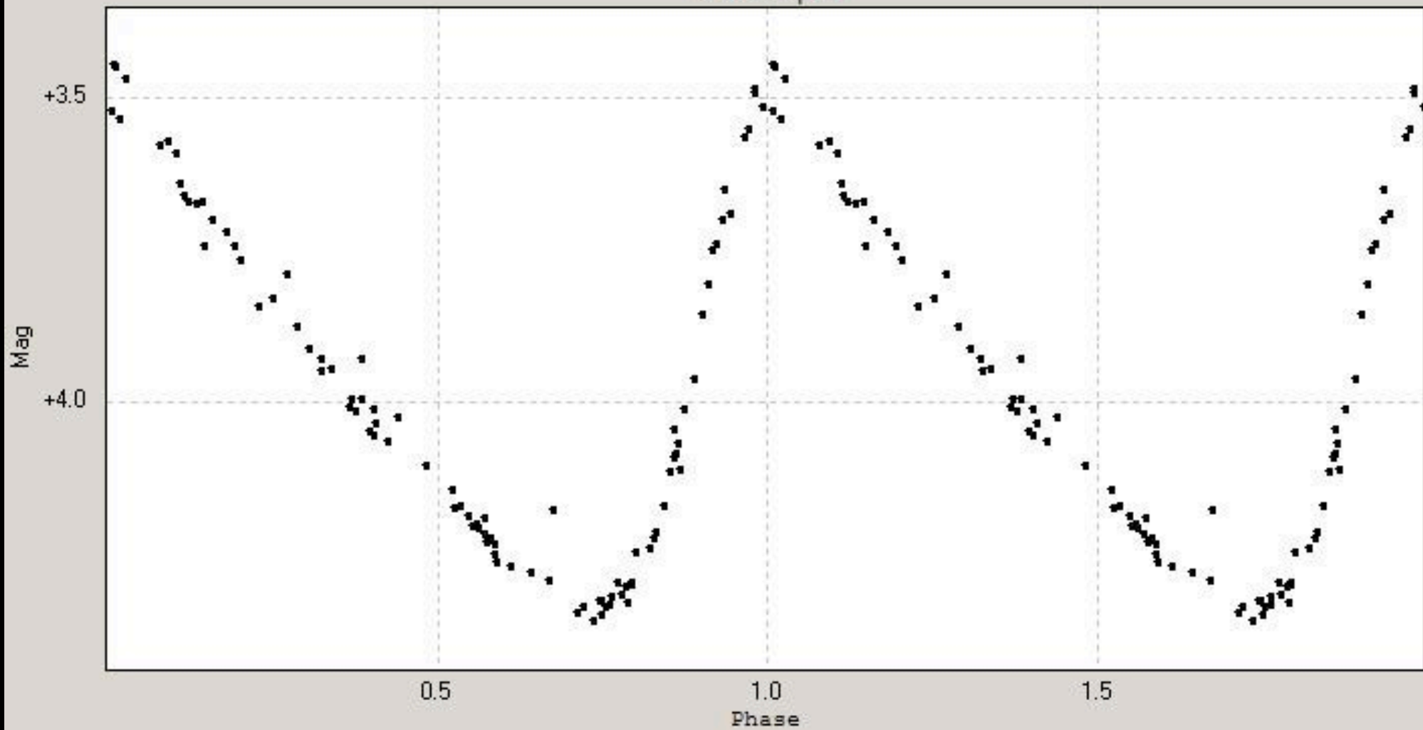
Delta Cephei
