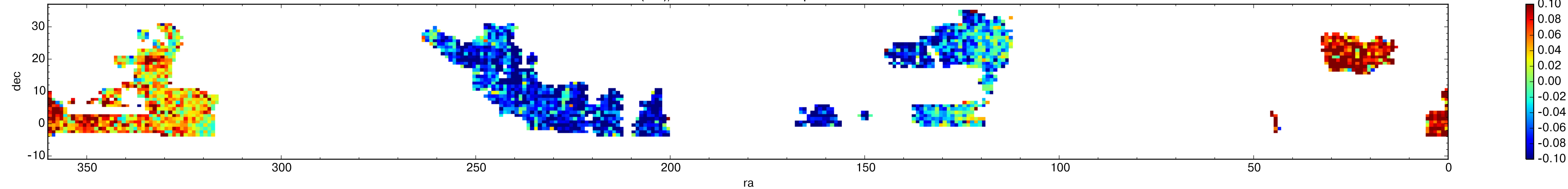
\delta(\text{Dec})/1 \text{ arcsec} for DR10 spec QSO
