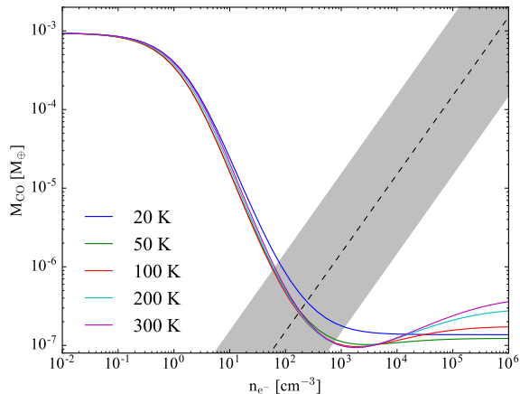
Figure 13. CO gas mass estimate of the detection at \sim 20 AU for different gas kinetic temperatures and electron densities ( n_{e^-} , main collisional partner). The dashed line corresponds to the CO gas mass assuming an abundance ratio of neutral carbon and CO of 100 and a carbon ionization fraction of 0.5. The shaded grey region represents a factor of 10 of uncertainty on the CO and electron abundance ratio.
