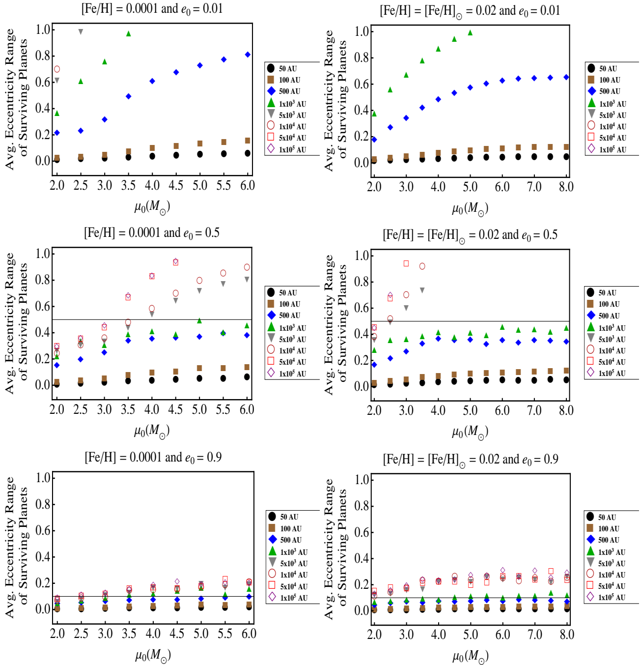
Figure 15. Eccentricity excitation of planets which remain bound during massive star evolution, for 2M_{\odot} - 8M_{\odot} . The left and right panels are for low metallicity and Solar metallicity, respectively. The top, middle and bottom panels are for e_0 = 0.01, 0.5 , and e = 0.9 , respectively. Each data point is averaged over the 50 values of the mean anomaly sampled for the given \mu_0 , a_0 , and e_0 values. If no symbol is displayed, then none of the corresponding systems were stable. The horizontal lines indicate values of 1 - e_0 ; symbols above this line experience a net eccentricity decrease.
