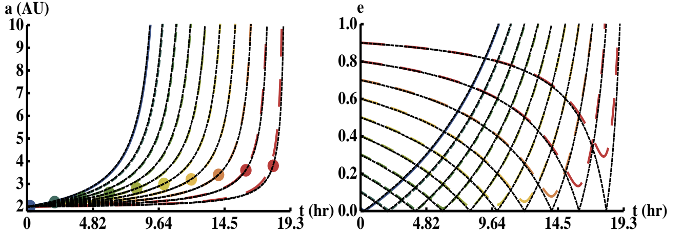
Figure 11. Analytic approximations (thin black nearly-solid foreground lines, from Eqs. 38, 41 and 44) to the e and a evolution from the numerical simulations (background-coloured dashed curves) in the same runaway regime as in Fig. 10, but for f_0 = 178^\circ . In the limiting case of f_0 = 180^\circ , the eccentricity decreases until reaching zero. The dots in the left panel indicate when this would have occurred (at a_0 [1 + e_0] ). None of the planets are ejected until at least half of the star’s mass is lost, and the highest eccentricity planets are not ejected until almost all of the star’s mass is lost (see Eq. 42).
