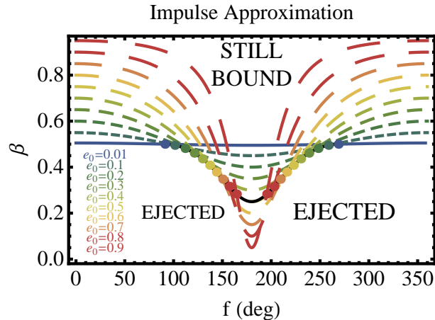
Figure 12. Ejection prospects in the impulse approximation ( \Psi_0 \rightarrow \infty ). Plotted is the fraction of stellar mass retained ( \equiv \beta ) vs. f_0 for 10 curves of increasing dash length for e_0 = (0.01, 0.1, 0.2, 0.3, 0.4, 0.5, 0.6, 0.7, 0.8, 0.9) . The planet remains bound in the regions above the curves and is ejected in the regions below the curves. The dots refer to the inflection points of the curves, given by Eq. (49) and which satisfy Eq. (23). Note how highly eccentric planets are especially protected from ejection near apocenter ( f \approx 180^\circ ), but are prone to ejection near pericenter ( f \approx 0^\circ ).
