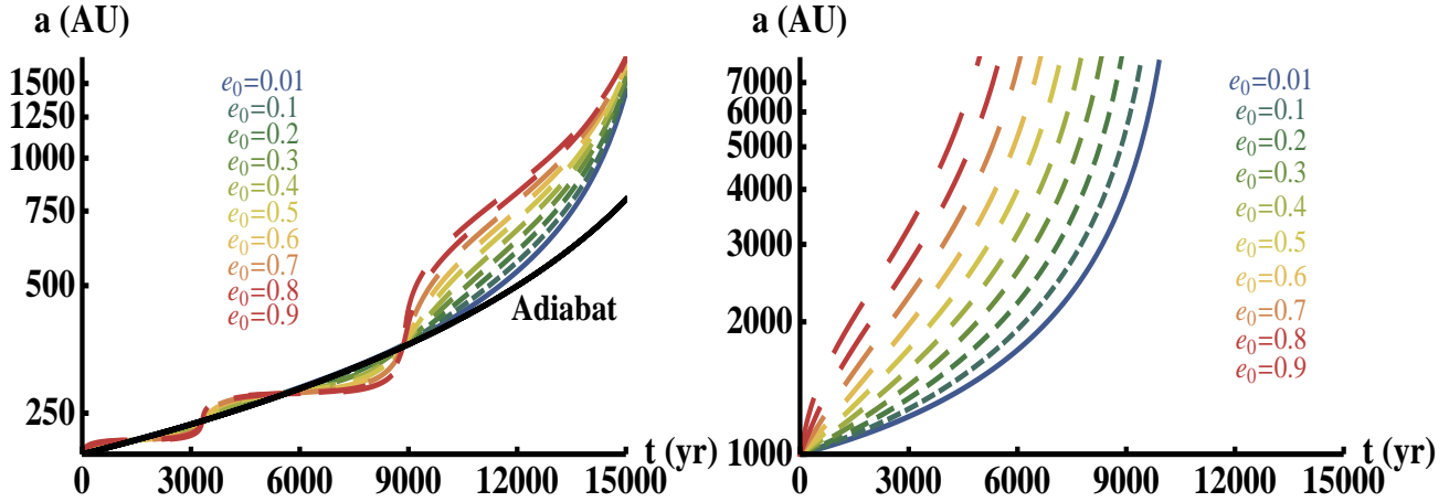
Figure 4. The breaking of adiabaticity for the same two systems in Fig. 3. In the left panel, note how the eccentric planets oscillate about the adiabat until reaching the runaway regime. In the right panel, the planets begin at t = 0 just off of the adiabat, and quickly settle into the runaway regime.
