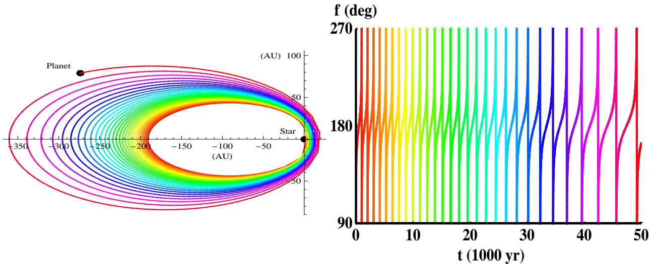
Figure 2. The adiabatic regime. The position in space ( left panel ) and the evolution of the true anomaly ( right panel ) of a planet (or belt particle) that is being pushed outward due to stellar mass loss. The colours on the curves indicate evolution at the same points in time, and the vertical lines of true anomaly indicate circulations of the angle. The star has an initial mass of \mu_0 = M_\star = 1M_\odot and is losing mass at the rate of \alpha = 1 \times 10^{-5} M_\odot/\text{yr} . The planet begins on a highly eccentric orbit ( e_0 = 0.9 ) at a_0 = 100 AU, with f_0 = 0^\circ . Hence, \Psi_0 = 0.0016 . Notice that as the planet moves outward and its mean motion decreases, the circulation period of the true anomaly decreases as well.
