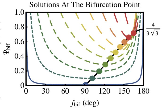
Figure 6. Values of (\Psi_{\text{bif}}, e_{\text{bif}}, f_{\text{bif}}) at the bifurcation point, where lines with increasing dash length represent e_{\text{bif}} values of 0.01, 0.1, 0.2, 0.3, 0.4, 0.5, 0.6, 0.7, 0.8, and 0.9, respectively. Corresponding colour dots represent the value of \Psi_{\text{bif,min}} for a given e_{\text{bif}} , when just one value of f_{\text{bif}} satisfies Eq. (22). Adiabatic systems approaching the bifurcation point would be traveling upwards on this plot while circulating nearly parallel to the X axis.
