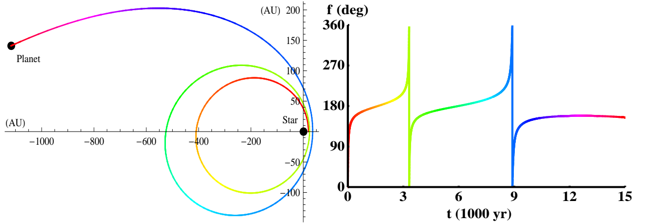
Figure 5. The position in space ( left panel ) and the evolution of the true anomaly ( right panel ) of the e_0 = 0.9 planet from the system in the left panels of Figs. 3 and 4. At t \approx 1.2 \times 10^4 yr, the planet stops circulating and starts to head out of the system as the true anomaly becomes stationary.
