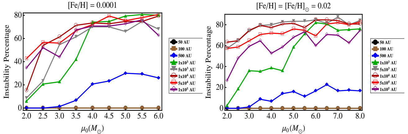
Figure 14. Planetary ejection prospects for massive stars from 2M_{\odot} - 8M_{\odot} . Each data point is averaged over the 150 randomly chosen mean anomaly values and 3 selected e_0 values for each a_0 . The black filled-circle curves for 50 AU are hidden behind the 100 AU curves. The a_0 = 50 and a_0 = 100 AU systems, which are in the adiabatic regime, remain bound. The a_0 \geq 10^3 AU systems, in the runaway regime, become largely unstable.
