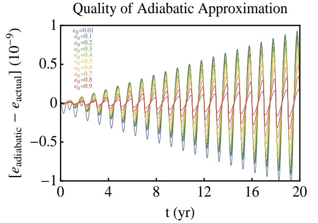
Figure 1. Analytic approximation to the eccentricity evolution in the adiabatic regime. Shown here is the difference in eccentricity of a planet evolving according to Eq. (17) compared to Eqs. (3)-(7). The planet is located at a_0 = 1 AU from a \mu_0 = 1M_\odot star which is losing mass at the rate of \alpha = 10^{-5}M_\odot/\text{yr} ( \Psi_0 \approx 1.6 \times 10^{-6} ). The differently coloured lines from the top of each crest moving downward correspond to e_0 = 0.01, 0.1, 0.2, 0.3, 0.4, 0.5, 0.6, 0.7, 0.8, and 0.9 respectively.
