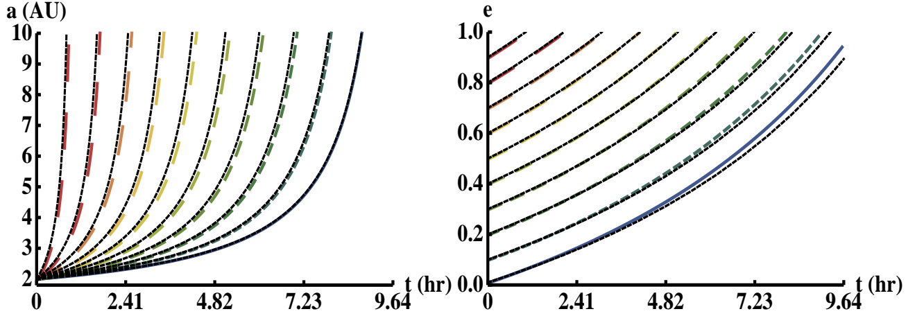
Figure 10. Analytic approximations (thick black nearly-solid foreground lines, from Eqs. 37 and 43) to the e and a evolution from the numerical simulations (background-coloured dashed curves) in a robustly runaway regime for f_0 = 20^\circ . The planet at a_0 = 2 AU is experiencing supernova-like mass loss of \alpha = 0.5M_\odot/\text{hour} from a \mu_0 = 10M_\odot star ( \Psi_0 \approx 62.4 ). The lines with increasing dash length represent e_0 values of 0.01, 0.1, 0.2, 0.3, 0.4, 0.5, 0.6, 0.7, 0.8, and 0.9, respectively. The analytical approximation is best for e_0 = 0.01 , and reproduces all the e_0 curves from the full numerical integrations to within 10%. All the planets are ejected before half of the star’s mass is lost (see Eq. 39).
