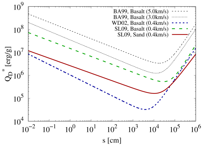
Figure B1. Q_D^* as function of size. The thin black dashed and dotted line show values for basalt at 3 and 5 km/s taken from Benz & Asphaug (1999). The parameters of the HD 109085 system are assumed. The thick blue dash-dotted line shows the scaling result taken for Wyatt & Dent (2002) and the thick green dashed line the lab results taken from Stewart & Leinhardt (2009) for basalt at 0.4 km/s. The thick solid red line shows the result for “sand” at 0.4 km/s taken from Stewart & Leinhardt (2009).
