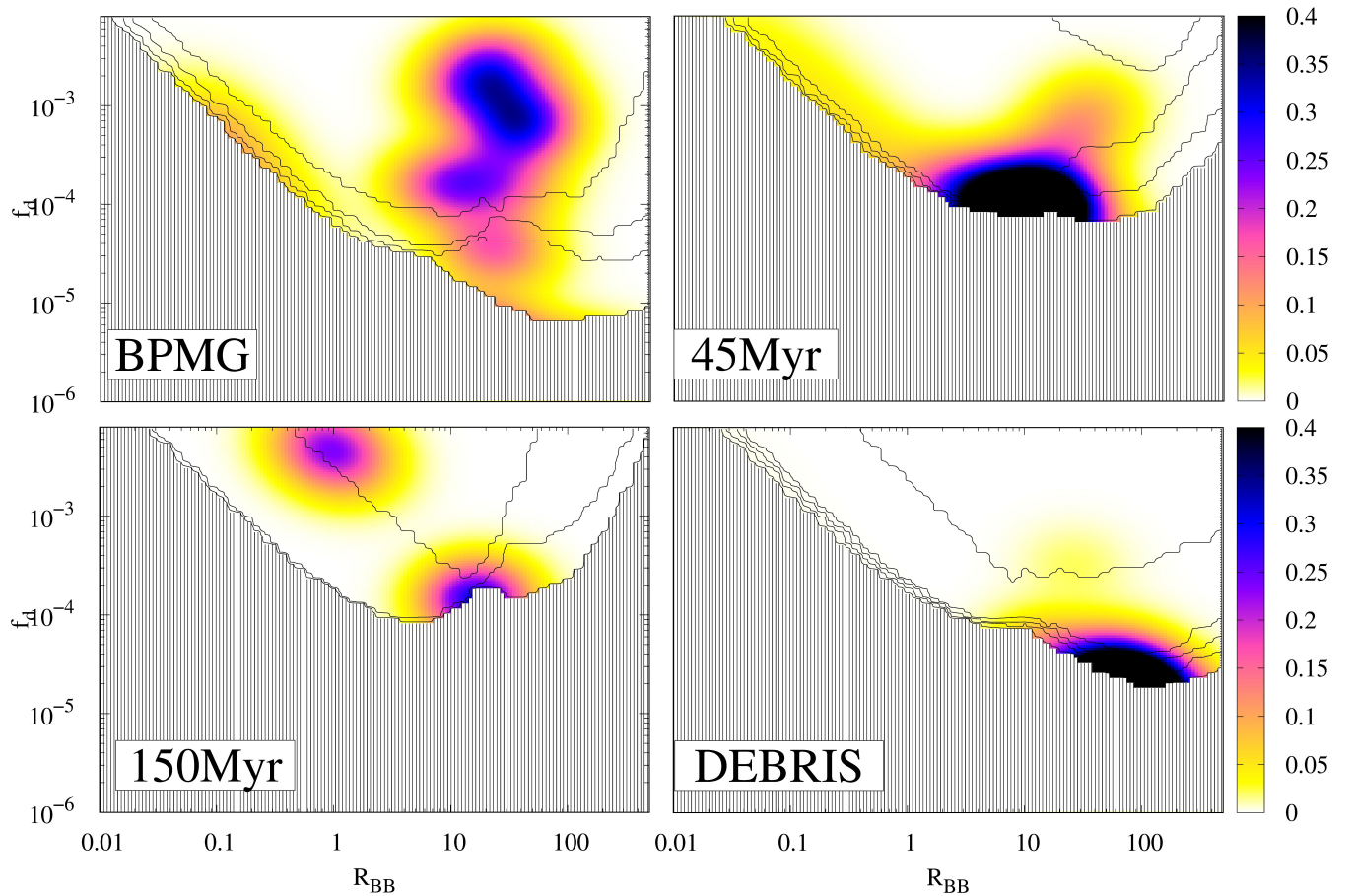
Figure 6. Fractional luminosity as function of blackbody radius for the four samples (BPMG, 45 Myr group, 150 Myr group, and DEBRIS). The colour scale shows the disc incidence, per \log(\text{au}) , per \log(\text{unit } f_d) . The contour lines show the levels of completeness for 0.1, 0.3, 0.5, 0.7 and 1.0 starting from the bottom of the plot.
