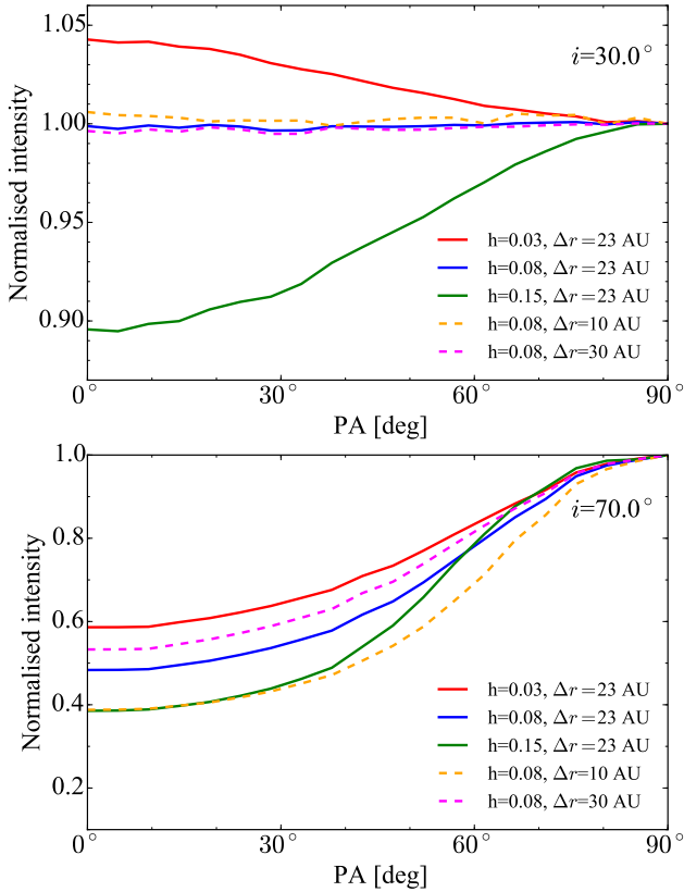
Figure 10. Intensity profiles along the ring projected ellipse on sky obtained from simulated Clean images without noise and using our best fit ring model. The values are normalised to the intensity at the ring semi-major axis (PA=90°). The upper panel corresponds to a disc inclined by 30°, while the lower to 70°. In red, blue and green lines we present three different profiles for disc aspect ratios of 0.03, 0.08 and 0.15 with \Delta r fixed to 23 AU, while in dashed lines we present profiles varying h and \Delta r .
