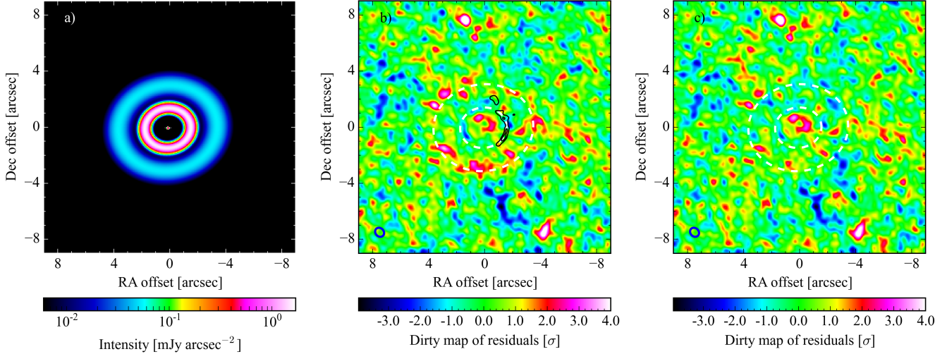
Figure 9. a) Synthetic model image of the best fit model with two rings at 220 GHz. b) Dirty map of the residuals of the best fit model with a single ring corresponding to natural weighting. The black contours represent the optical depth deviations from a uniform disc derived from HST images (Stark et al. 2014, left panel Figure 1). c) Dirty map of the residuals of the best fit model with two rings corresponding to natural weighting. The white dashed contours in panels b) and c) correspond to radius of the main and second ring of the best fit two rings model. The Clean beam is represented by a blue ellipse ( 0''.67 \times 0''.58 ) in the bottom left corner. The x- and y-axes indicate the offset from the stellar position in R.A. and decl. in arcsec, i.e. north is up and east is left.
