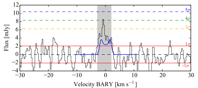
Figure 8. Blue line: model spectrum. Black line: continuum subtracted integrated spectrum inside an elliptic mask of minimum and maximum semi-major axis of 1''.4 and 2''.1 , and oriented as the dust continuum ring. The horizontal lines represent \pm 1 , 3, 4 and 5\sigma levels. The grey region represents velocities between -2.8 \text{ km s}^{-1} and 2.0 \text{ km s}^{-1} . The velocities represent the Doppler shift with respect to 230.538 \text{ GHz} in the Barycentric reference frame.
