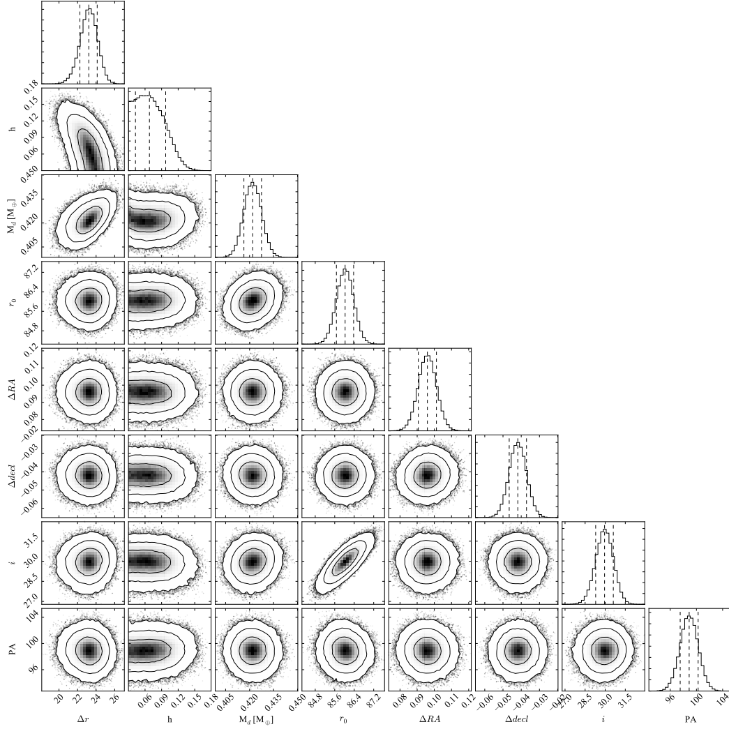
Figure A1. Posterior distribution of \Delta r , h = H/r , M_d , r_0 , RA and decl offsets, i and PA. The 1D marginalised distributions are presented in the diagonal, while the 2D marginalised distributions are presented in the bottom left half. The vertical dashed lines represent the 16th, 50th and 84th percentiles. Contours correspond to 68%, 95% and 99.7% confidence regions and the black dots to points of the MCMC outside the 99.7% confidence region. This plot was generated using the python module corner (Foreman-Mackey et al. 2014).
