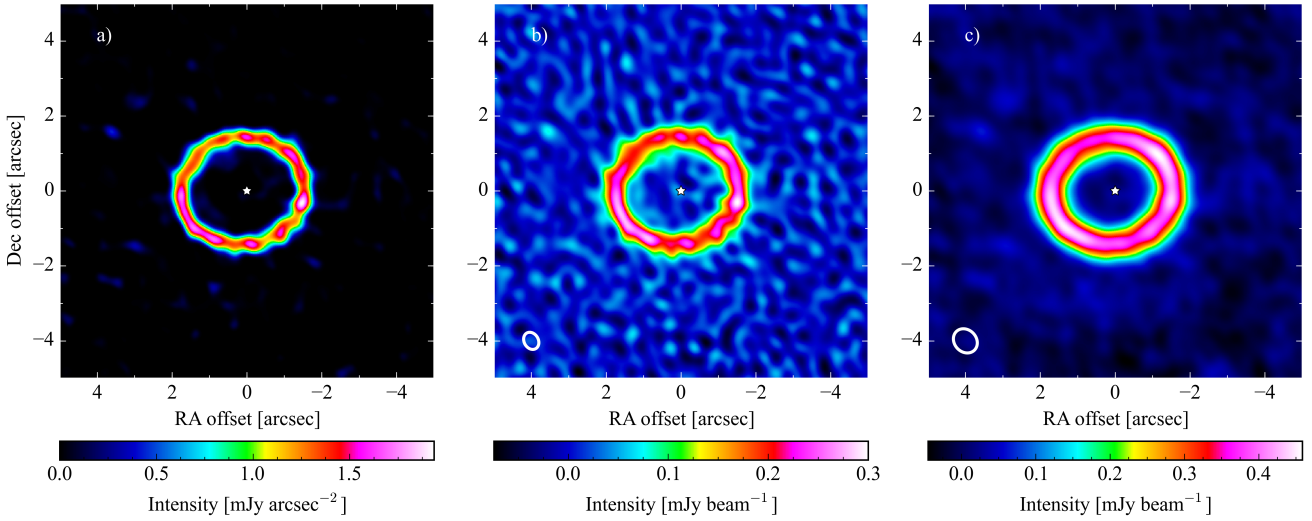
Figure 1. ALMA dust continuum maps at 220 GHz (Band 6). a) MEM non-parametric model (regularized with the maximum entropy method). b) Restored image adding residuals and convolving with a synthetic beam corresponding to Briggs weighting ( 0''.47 \times 0''.36 ). c) Restored image adding residuals and convolving with a synthetic beam corresponding to natural weighting ( 0''.69 \times 0''.58 ). The respective beams are represented by white ellipses. The x- and y-axes indicate the offset from the stellar position in R.A. and decl. in arcsec, i.e. north is up and east is left. The stellar position is marked with a white star.
