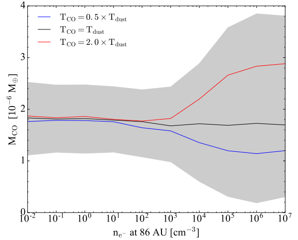
Figure 6. Best fit CO gas mass values obtained from our MCMC analysis using different kinetic temperatures and electron densities ( n_{e^-} , main collisional partner). The blue, black and red lines correspond to kinetic temperatures equal to 0.5, 1 and 2.0 times the dust temperature in the disc, respectively. The grey area represents the 68% confidence region with gas temperatures ranging between 0.5 – 2.0 times the dust temperature.
