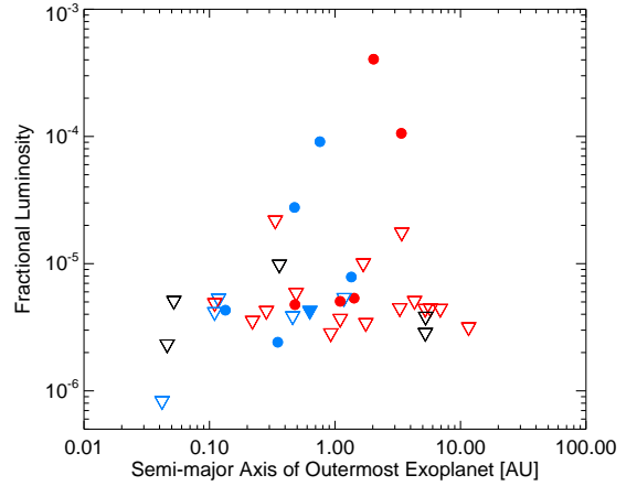
(f) Semi-major axis of outer exoplanet's orbit vs. fractional luminosity.
