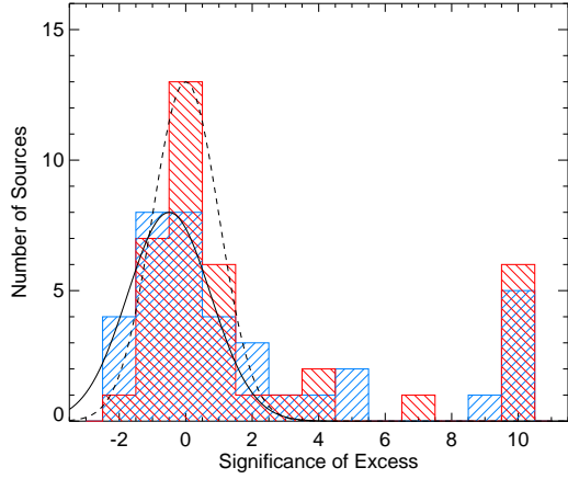
Fig. 1. Histogram plot of the distribution of the significances presented in Table 2 at 100\ \mu\text{m} (in blue, hatching top right to bottom left) and 160\ \mu\text{m} (in red, hatching top left to bottom right). Debris disc stars with \chi values greater than ten have been added to the right hand side bin.
