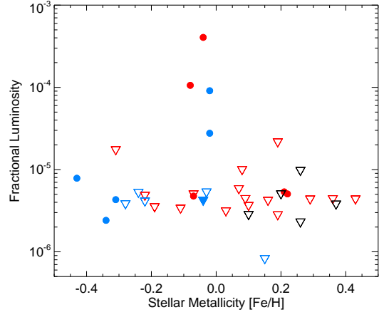
(b) Metallicity vs. fractional luminosity.
