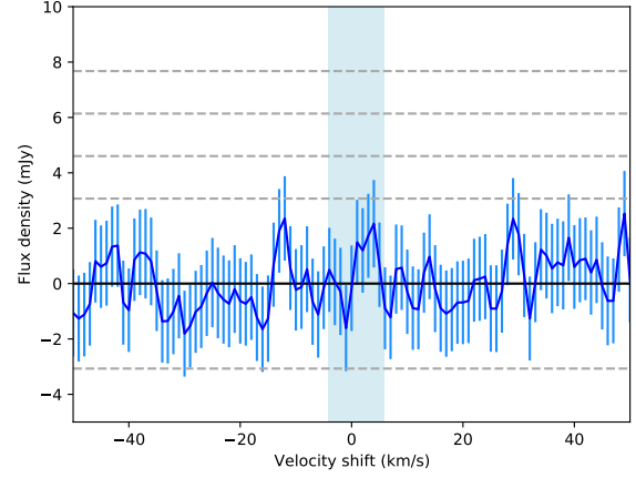
Figure 2. ALMA CO spectrum centred on a rest frequency of 230.538 GHz. The blue shaded region denotes the 10 km/s wide channel used to determine the presence of CO emission, centred on the stellar velocity. Uncertainties are 1\text{-}\sigma . The grey dashed lines denote uncertainties from \pm 2\sigma in steps of 1\text{-}\sigma .
