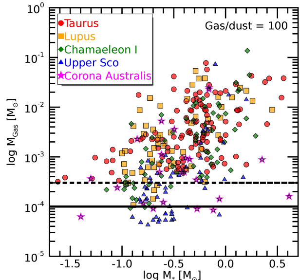
Figure 2. Distribution of disk masses as a function of the stellar mass for nearby star forming regions, based on recent millimeter dust continuum observations with the SMA and ALMA (Andrews et al., 2013; Ansdell et al., 2016; Barenfeld et al., 2016; Pascucci et al., 2016; Cieza et al., 2019; Cazzoletti et al., 2019) and assuming a global gas-to-dust mass ratio of 100. The two horizontal lines indicate the detection limits that will be achieved with SAFARI observations of the HD J = 1 - 0 line fluxes in the case of the shallow (1 h on-source, dashed line) and deep (10 h on-source, dotted) surveys, following the HD line flux predictions from Trapman et al. (2017).
