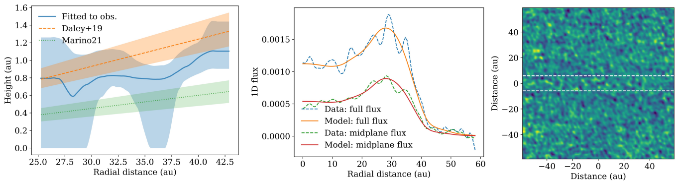
Figure 11. This figure shows the fitted scale height and range of possible models assuming an inclination of 88.5^\circ . The full 1D flux and midplane flux of the observation and the best-fit model are displayed in the middle panel. The right panel shows the residual image obtained by subtracting the best-fit model from the data. A dashed box locates the approximate spatial extent of the disk.
