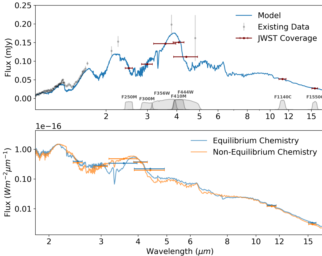
Figure 2. Top panel: The spectral coverage of HIP 65426b we will achieve using NIRCam and MIRI Coronagraphy (red points), compared to the existing VLT-SPHERE and NACO photometric points (Cheetham et al. 2019) shown in black/grey, and overlaid with a model ( T_{\text{eff}}=1340 K, \log(g)=3.95 ) computed using the tools described in Tremblin et al. (2015). The simulated JWST data points reflect the integral of the flux density over the filter bandpass, divided by the width of the bandpass. Bottom panel: Two example synthetic atmosphere models (assuming the same physical parameters for each model) taken from Phillips et al. (2020) illustrating the effects of non-equilibrium chemistry (orange curve) compared to equilibrium chemistry (blue). Also shown are the photometric points from NIRCam and MIRI we will obtain, which will easily have the precision to differentiate between the two models, particularly at 3.56 \mu\text{m} .
