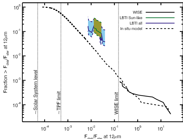
Figure 7. Exozodi luminosity function constrained by our LBTI statistics and the WISE sample by Kennedy & Wyatt (2013). Occurrence rates and sensitivities for Sun-like and all stars are consistent, so that the two curves lie on top of each other. The slope from the WISE detection rate to the one from the LBTI appears steeper than the prediction from the in situ dust production model by Kennedy & Wyatt (2013).
