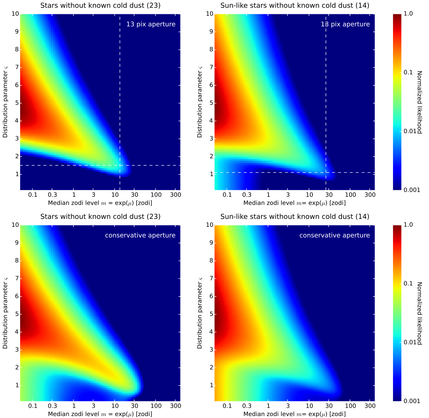
Figure 3. Likelihood distribution of our fits of a lognormal luminosity function to the observed zodi levels and uncertainties from Table 2 for all clean stars ( left ) and all clean Sun-like stars ( right ). A 1/m prior on the median m = \exp(\mu) is applied, equivalent to assuming a flat prior for the lognormal parameter \mu . The top row shows the results from the zodi levels derived from the 13 pix aperture, while the bottom row shows those derived from the conservative aperture. There are no inconsistencies between the results derived from the two apertures other than the weaker constraints for the conservative aperture due to the larger uncertainties of the individual measurements. The white, dashed lines in the plots for the 13 pix aperture indicate our 95% confidence interval on m and the corresponding best-fit of the sigma parameter of the lognormal luminosity function. These are our current recommendations for the exozodi distribution to use for estimating yields for future exo-Earth imaging missions (Sect. 6.2).
