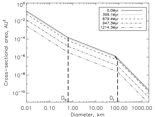
Figure 9. Evolution of the size distribution for an initial transition diameter of 70 km and initial mass of 40 M_{\odot} . The size distribution continues down to D_{bl} but this has not been shown for clarity. The thick dashed lines represent the break diameter and the transition diameter. There is some increase in D_t pre-LHB when mass is being lost through collisions but the size distribution then remains fixed from the onset of the LHB and all the mass lost after this time is due to dynamics.
