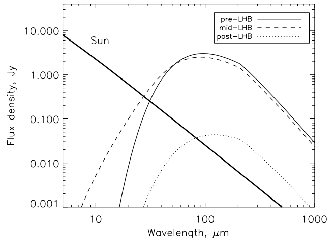
Figure 3. SED before, during and after the LHB, as it would appear from 10 pc away. The thick line shows the solar photosphere. The thin lines show the excess emission at 873 Myr, 881 Myr and 1212 Myr. The total emission spectrum observed would be the sum of the photosphere and excess.
