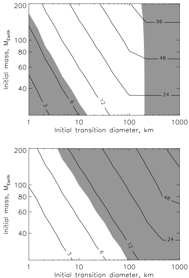
Figure 10. Dependence of mass at the time of the LHB on the initial conditions. Contours show the mass in Earth masses and the shaded regions represent runs that give a final transition diameter smaller or larger than the current constraints on the present day transition diameter. The runs shown in the top plot use the Löhne et al. (2008) Q_{\text{D}}^* and q_p = 2.2 and those in the bottom plot use the Leinhardt & Stewart (2009) Q_{\text{D}}^* and q_p = 2.2 .
