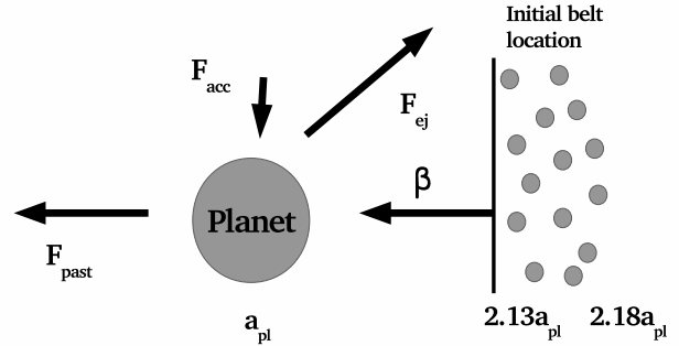
Figure 1. A schematic diagram of our approach, indicating the location of the initial belt in the N-body simulations which track the fraction of particles ejected by the planet ( F_{ej} ), the fraction accreted by the planet ( F_{acc} ) and the fraction that migrate past the planet, going on to hit the star ( F_{past} ), as described in §2.
