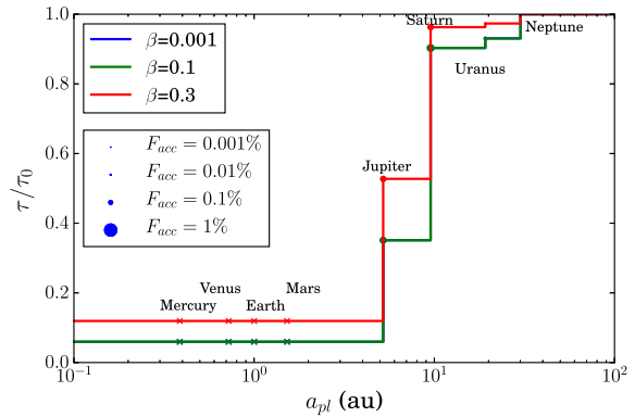
Figure 11. The change in effective optical depth of dust migrating inwards via PR-drag from the Kuiper belt, as it encounters the Solar System planets. The empirical model (Eq. 17 20 21 22) with best-fit parameters from Table 1 is used to calculate the fraction of dust ejected or accreted by each planet in turn. Collisional depletion is ignored. The fraction of the dust that approaches each planet that is accreted is shown by the size of each marker at the position of each planet.
