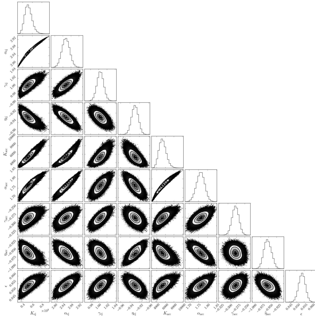
Figure 4. The posterior probability distributions of each parameter in the empirical fit to the ejections and accretions seen in the N-body simulations (Eq. 4, 20, 17), calculated by maximising the likelihood (Eq. 23). Plot created using corner from Foreman-Mackey (2016).
