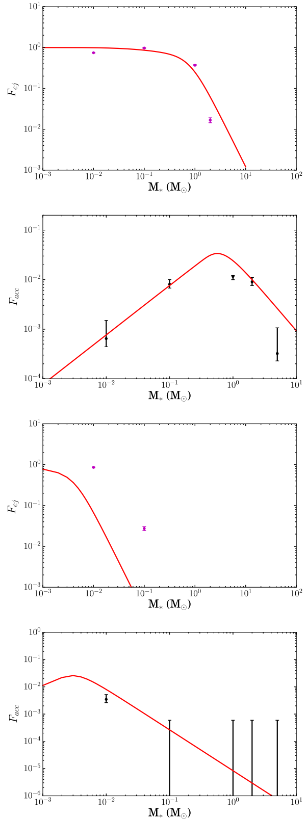
Figure 8. The fraction of particles ejected and accreted in the numerical simulations for M_{pl} = 100M_{\oplus} (top two plots), M_{pl} = 1M_{\oplus} (bottom two plots), \beta = 0.1 and a_{pl} = 1\text{au} , varying stellar mass ( M_* ), compared to predictions, based on Eq. 20, Eq. 17 using \delta_a = 1/2 and \delta_e = -5/2 , as described in §4.1.
