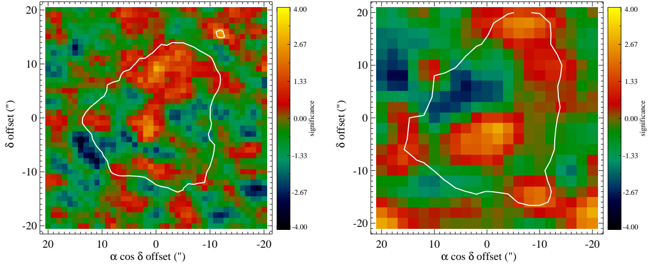
Figure 7. The residuals, in units of significance of (image-model)/uncertainty, from the model fits with a single belt described in §4.2 at 100 (left) and 160 \mu\text{m} (right). The models provide a good fit to the observations, the residuals are at low levels (note the scale), with the black contours showing residuals of 3 - \sigma . The white contours show the 3 - \sigma detection of the disc, as shown in Fig. 3 and Fig. 4.
